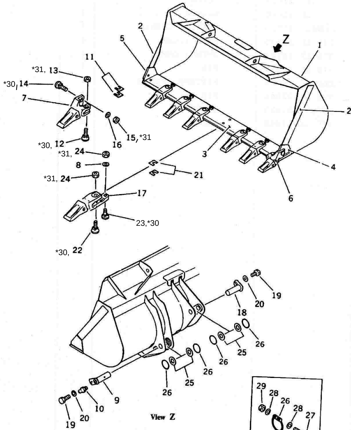
FIG 7010 BUCKET
