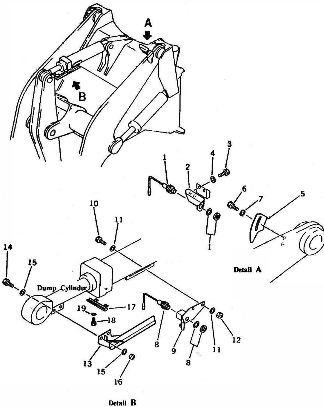
FIG 6100 BOOM KICK OUT AND BUCKET POSITIONER (OPTIONAL)
