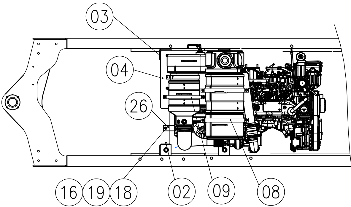
FIG 5050 EXHAUST SYSTEM
