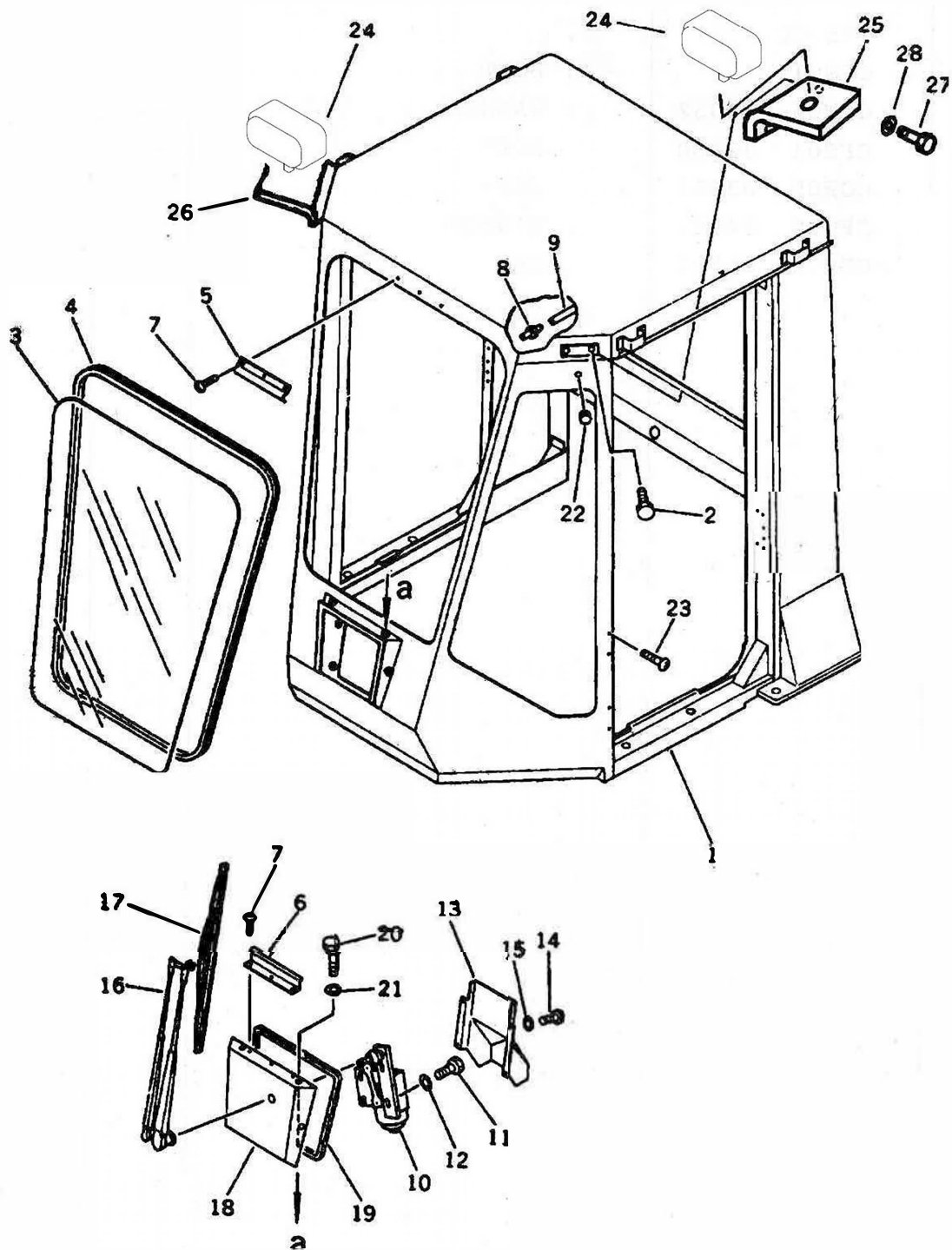
FIG 5110 CABIN ASSEMBLY (FRONT) (2/6)
