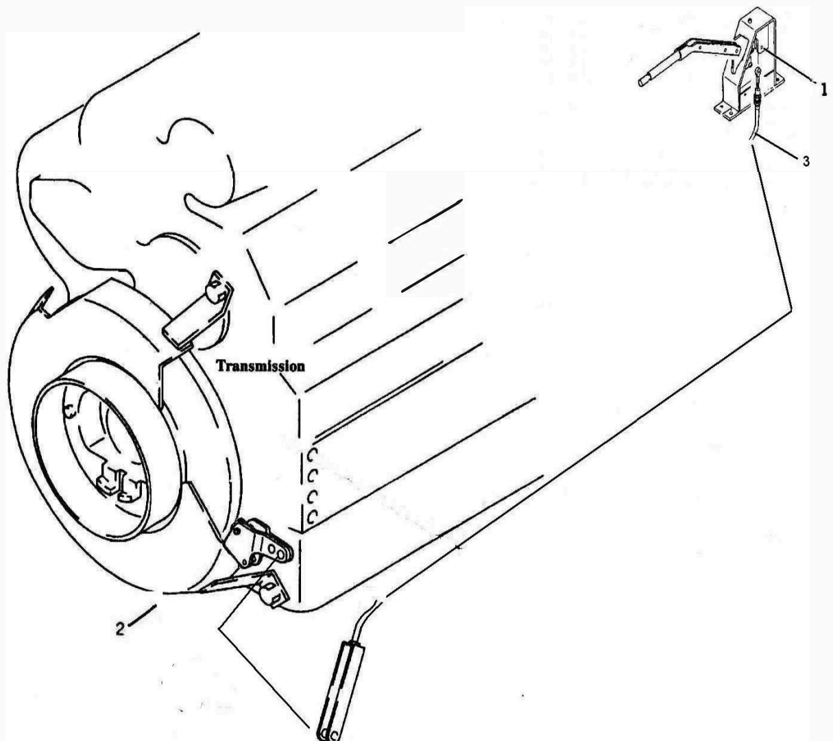
FIG 3040 PARKING BRAKE MOUNTING PARTS
