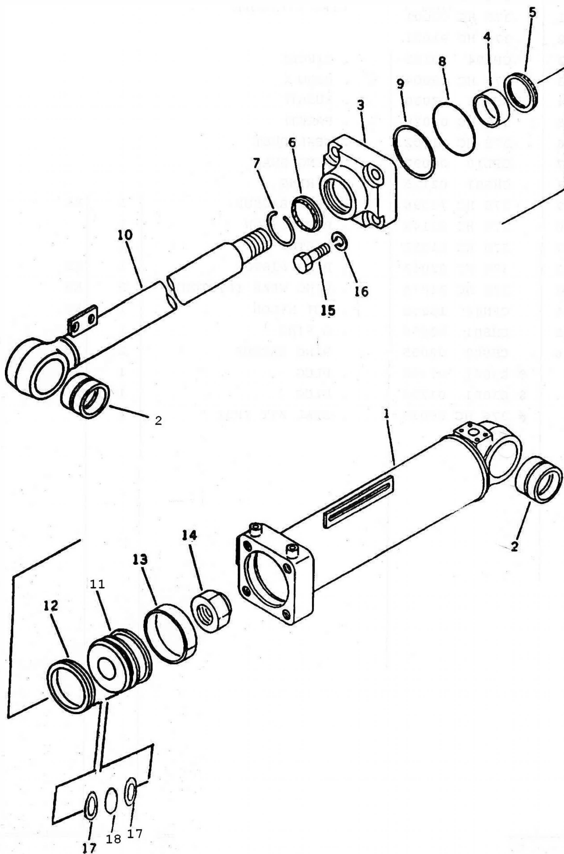
FIG 6040 DUMP CYLINDER
