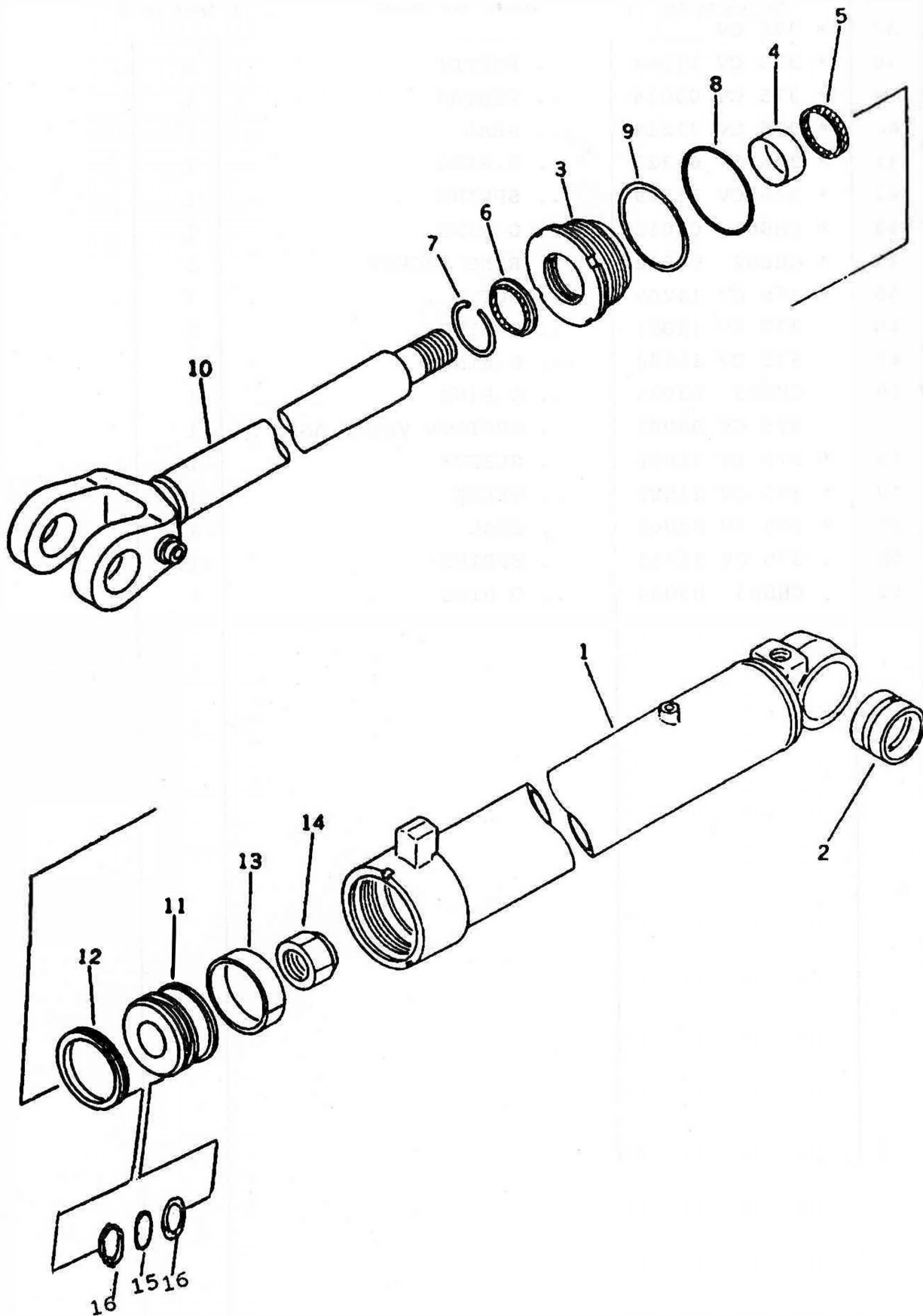
FIG 6030 LIFT (BOOM) CYLINDER
