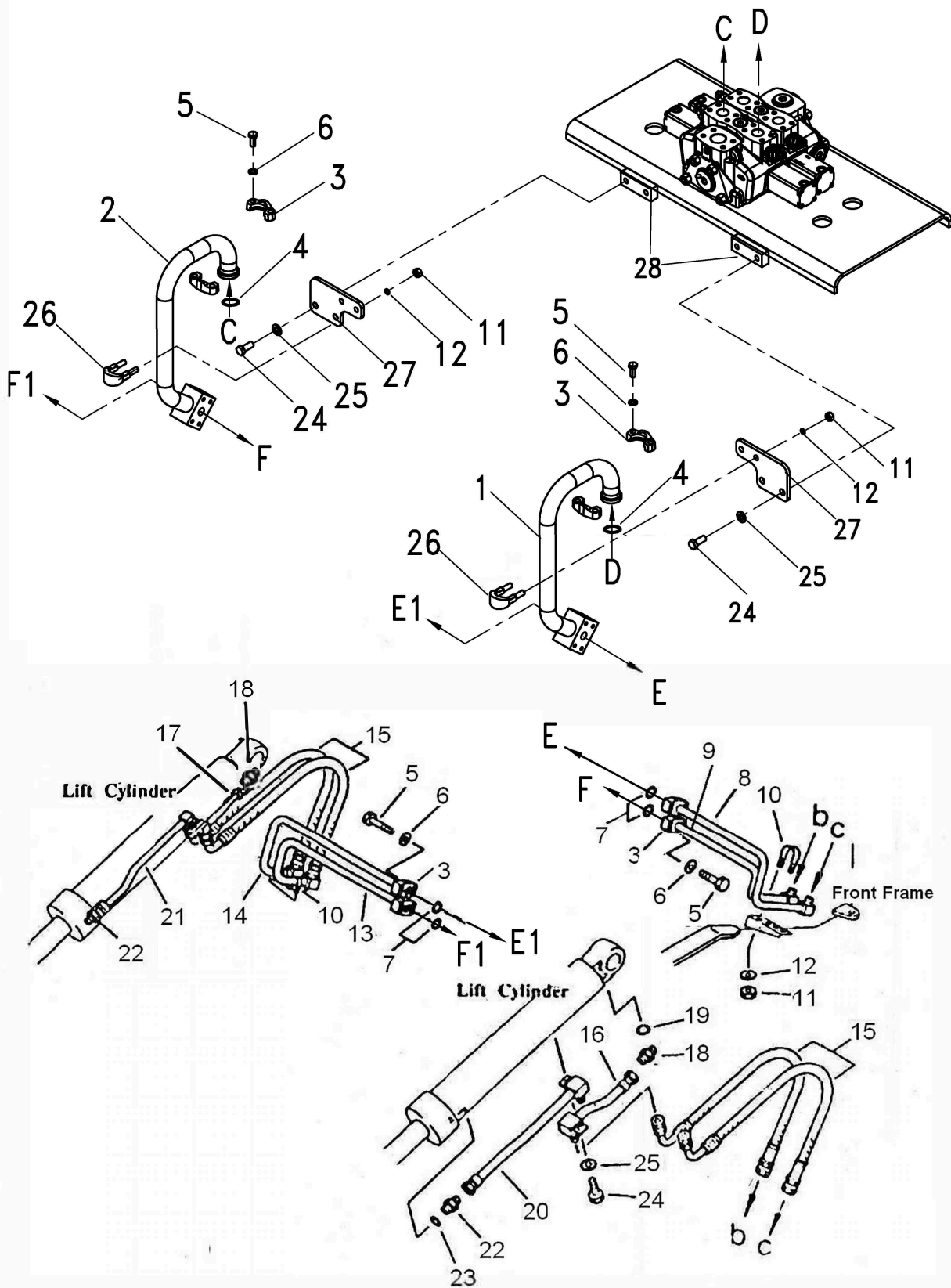
FIG NO 6060 HYDRAULIC PIPING (CV TO LIFT CYLINDER)
