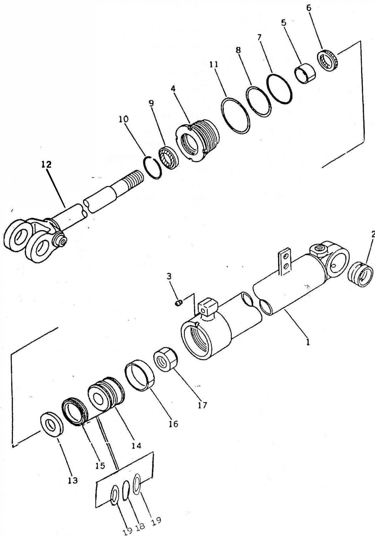
FIG 4020 STEERING CYLINDER
