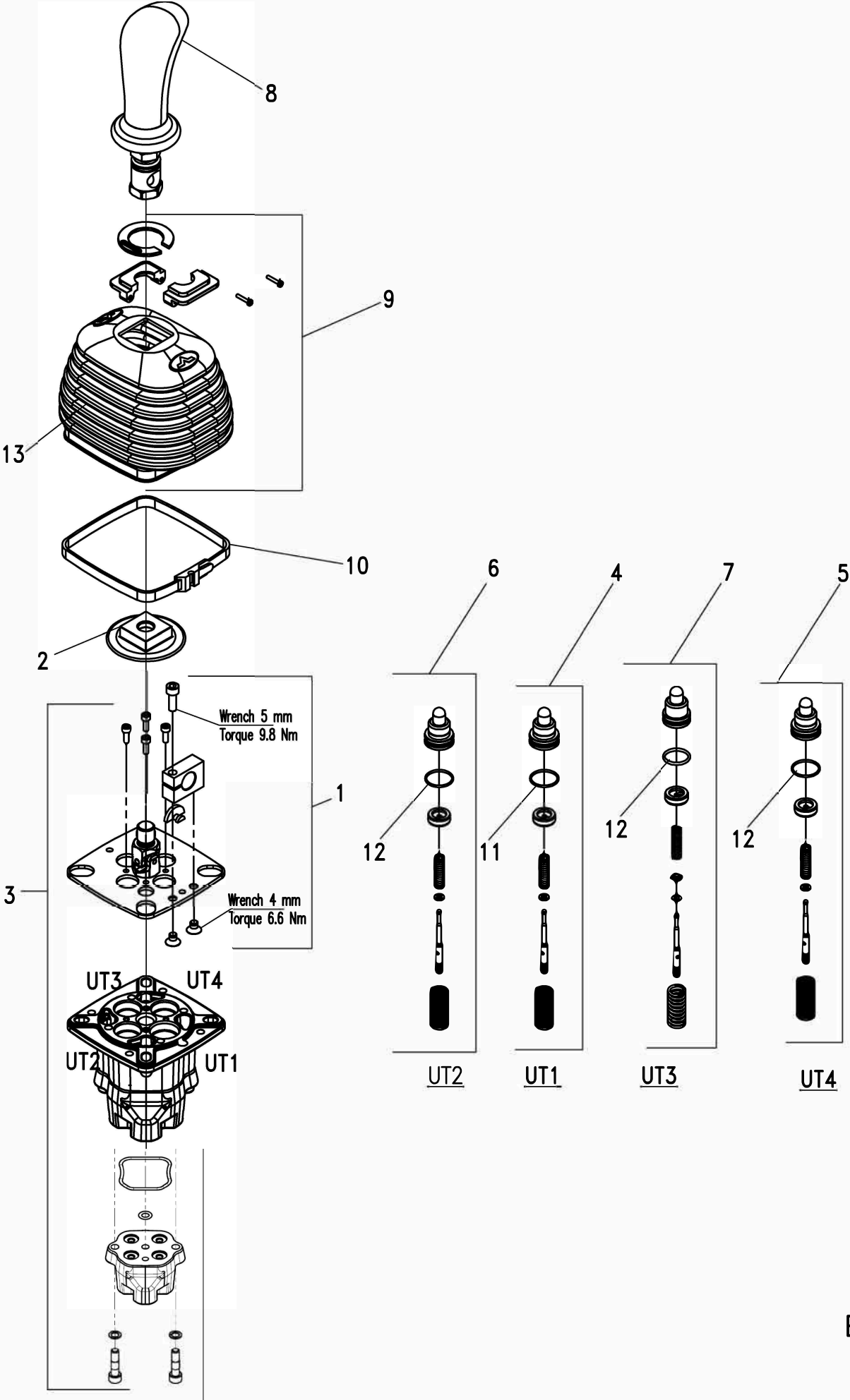
FIG 4050 JOYSTICK
